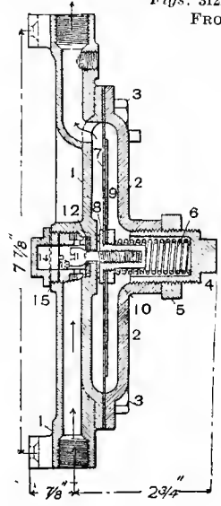
Fig. 3118. Cross Section.
